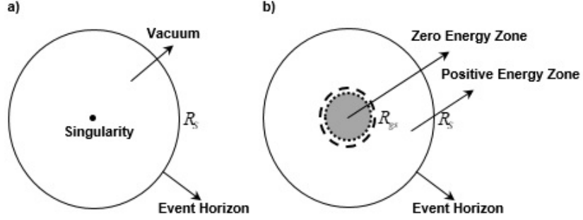
Figure 3: Internal structure of the black hole. a) Existing model b) New model. If, over time, the black hole stabilizes, the black hole does not have a singularity in the center, but it has a zero energy zone.
