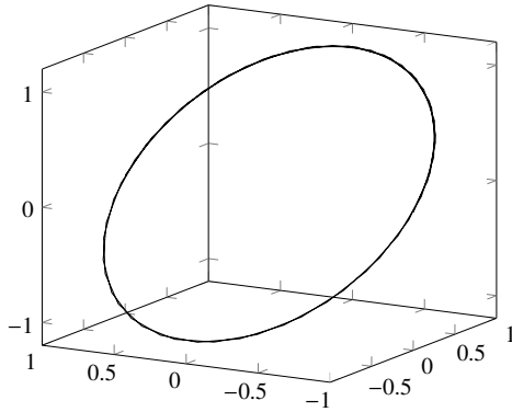
Fig. 18: Direction change graphic of the force applied, by the parametric curve of [\sin t, \cos t, \sin t, t, 0, 2\pi] . Magnitude of the force applied is the same at any point of the elips; so as force is applied by the same intervals at a fixed speed, the changing thing is displacement time around circumference of the elips.
