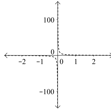
Fig. 7: f(t) function for x : 1 and y : 50 scale
