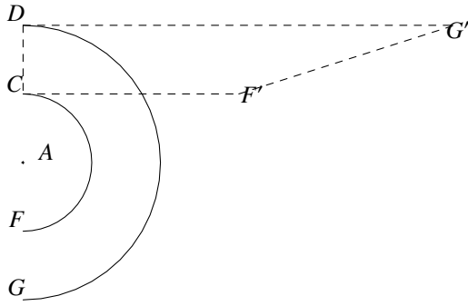
Fig. 32: The area of the circle in the kind of triangle
