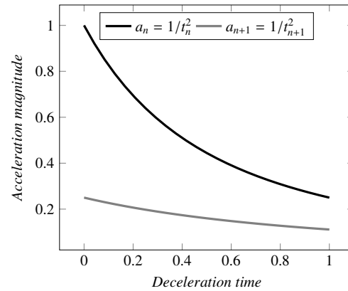
Fig. 3: Deceleration for a limited interval
