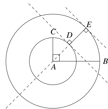
Fig. 31: The area scanned
