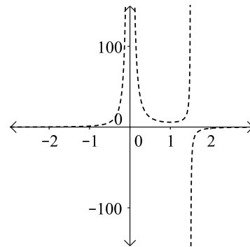
Fig. 8: a(t) function for x : 1 and y : 50 scale
