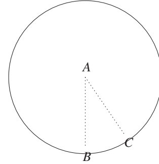
Fig. 37: Two points on the circumference
