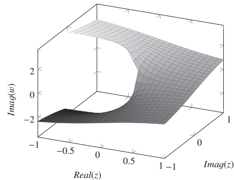
Fig. 31: Single branch of a random Riemann surface
