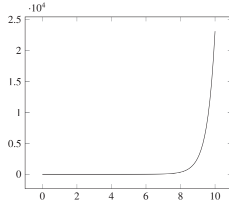
Fig. 36: Partial Palindromic prime separation
