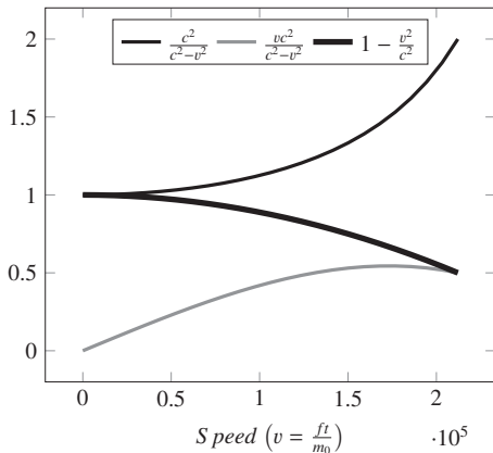
Fig. 32: Mass, length contraction and speed changing graphic from m = m_0 to m = 2m_0 , and L = L_0 to L = L_0/2
