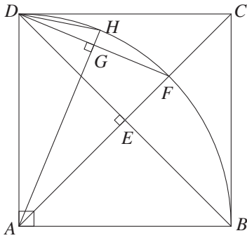
Fig. 42: The quarter slice of Fig. 41
