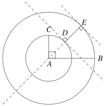
Fig. 43: The area scanned
