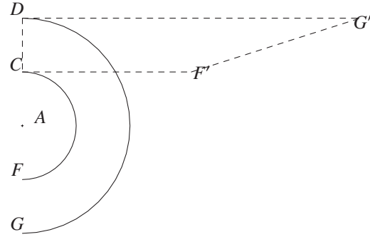
Fig. 44: The area of the circle in the kind of triangle
