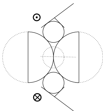
Fig. 47: The spherical balls
