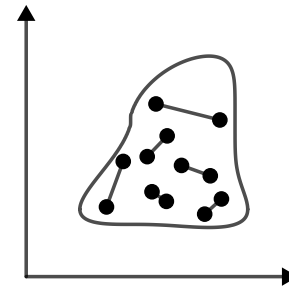
Fig. 25: Conservative area with a random closed curve
