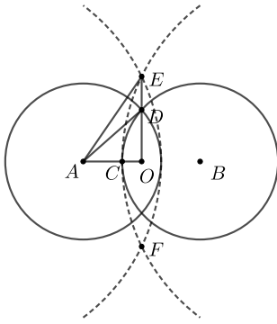
Fig. 35: Another representation of gravitational waves
