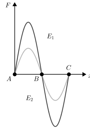
Fig. 45: Near gravitational waves
