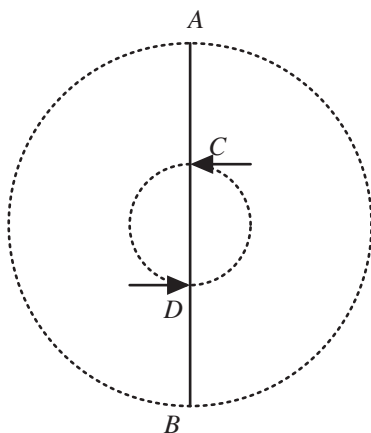
Fig. 48: An object which is about to go at light speed
