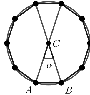
Fig. 27: Polygon transformation being n is even number
