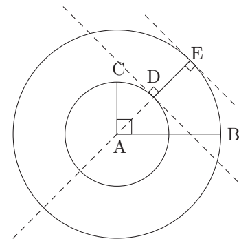
Fig. 47: The area scanned
