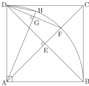
Fig. 46: The quarter slice of Fig. 45
