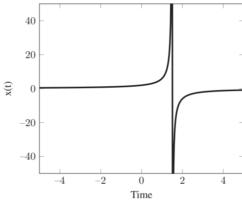
Fig. 10: x(t) function for x : 1 and y : 10 scale
