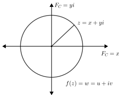
Fig. 29: Complex plane
