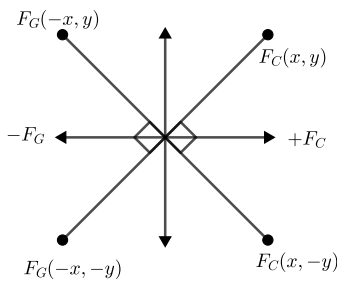
Fig. 28: Gravity and centrifugal force
