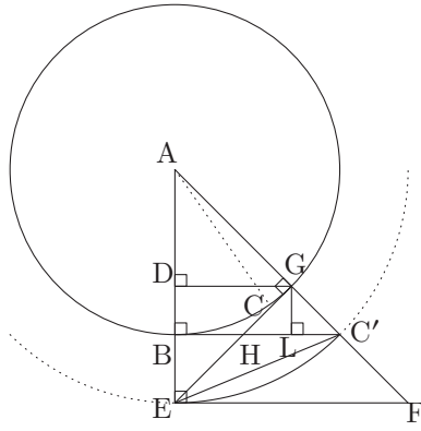
Fig. 43: The second radius
