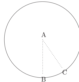
Fig. 41: Two points on the circumference
