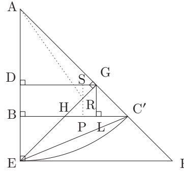
Fig. 44: A part of Fig. 43
