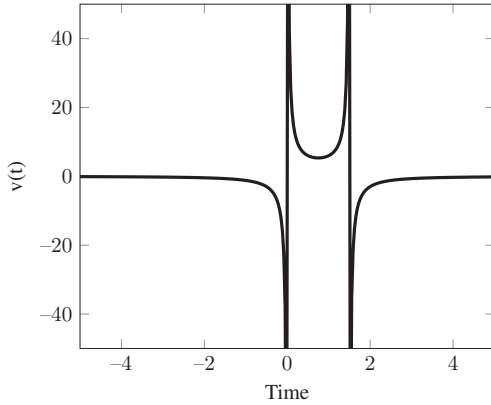
Fig. 9: v(t) function for x : 1 and y : 10 scale
