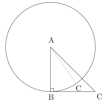
Fig. 42: The arc side
