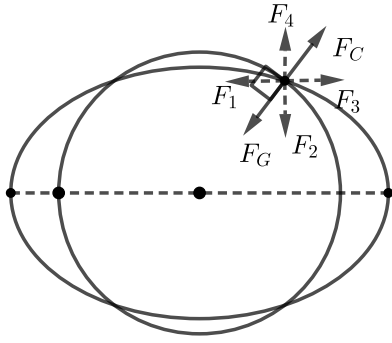
Fig. 36: Circular and elliptic orbits
