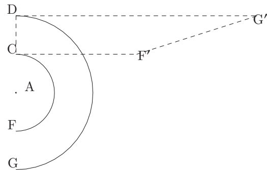
Fig. 48: The area of the circle in the kind of triangle
