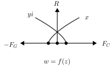
Fig. 30: Complex plane for the image set
