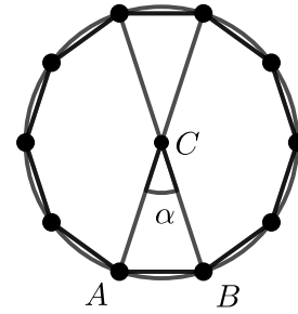
Fig. 27: Polygon transformation being n is even number
