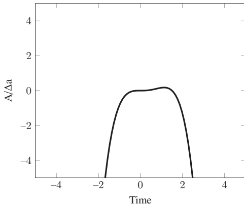
Fig. 6: A/Δa function
