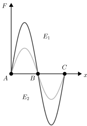
Fig. 38: Near gravitational waves
