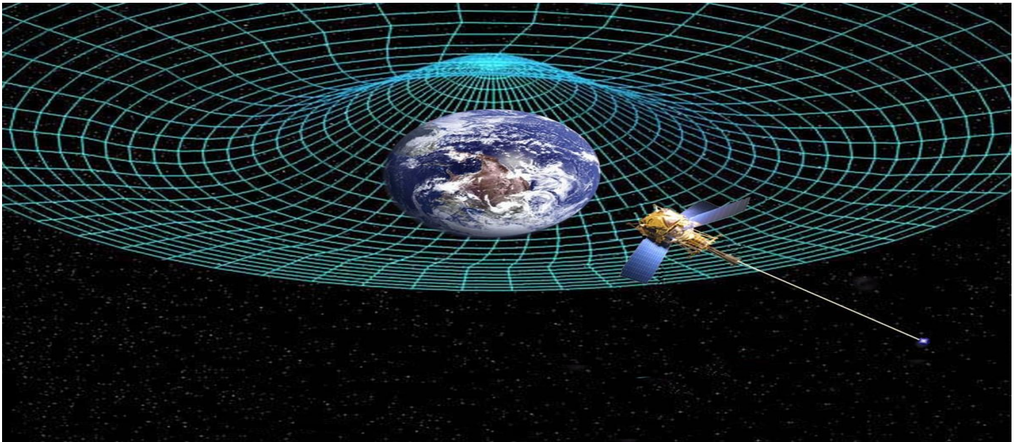
Fig 2 | visualization of how space distortion can explain repulsion. (Image: rotation of a © NASA image)
