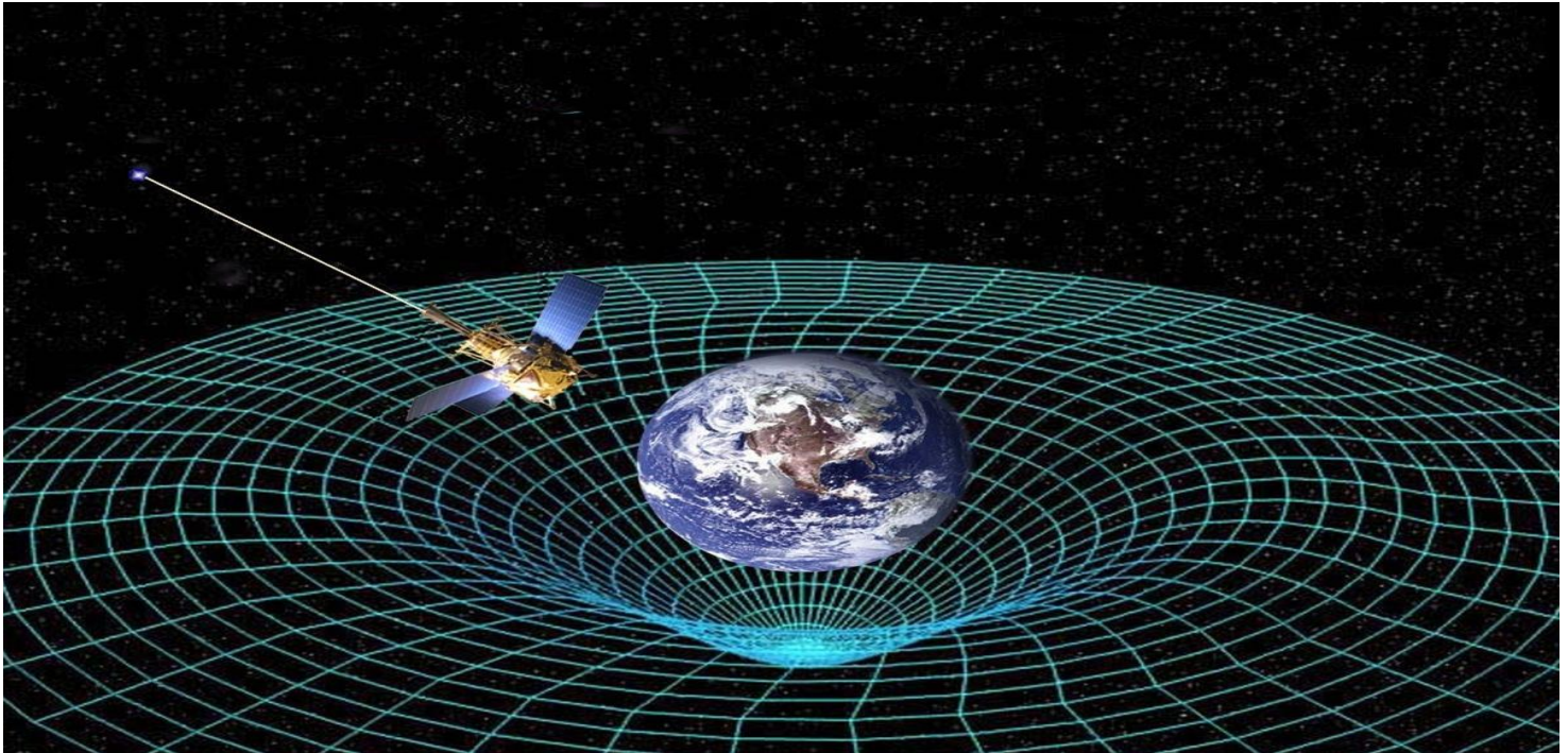
Fig 1 | visualization of how space distortion can explain attraction. (Image: © NASA)
