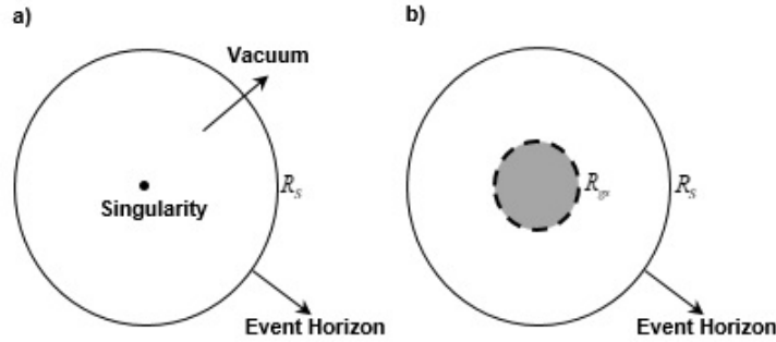
Figure 4: a) Existing Model. b) New Model. The area of within R_{gs} (or R_{gs-vir} ) has gravitational self-energy (potential energy) of negative value, which is larger than mass energy of positive value. If r is less than R_{gs} , this area becomes negative energy (mass) state. There is a repulsive gravitational effect between the negative masses, which causes it to expand again. This area (within R_{gs} ) exercises anti-gravity on all particles entering this area, and accordingly prevents all masses from gathering to r=0 . Therefore the distribution of mass (energy) can't be reduced to at least radius R_{gs} (or R_{gs-vir} ).
