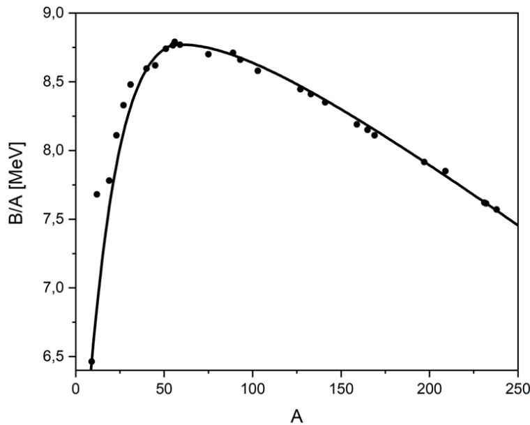
Figure 4. Binding energy/nucleon (MeV) as function of the nucleon number A . (●) experimental values; (—) calculated values with Equation (28).
