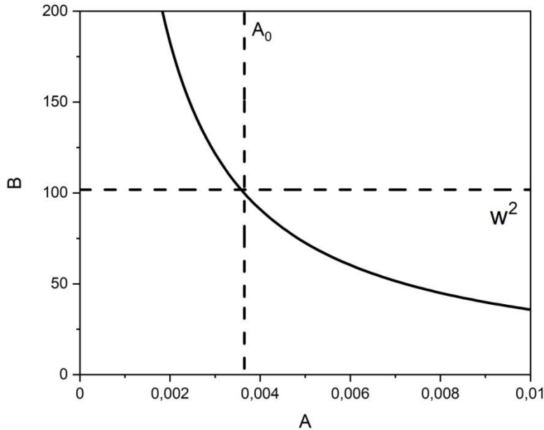
Figure 2. Graph of B = (1/e \cdot A) \cdot e^{e \cdot A} .
