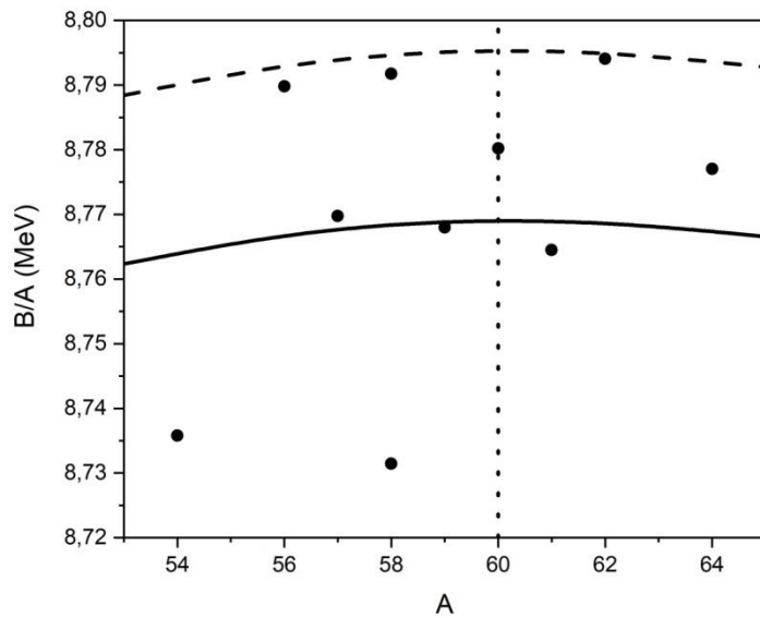
Figure 5. Binding energies B/A (●) obtained from atomic masses [13] for the 10 isotopes from Table 10 [13] and calculated (—) with Equation (27). Calculated (- - -) values with B/62 = 8.794 for ^{62}\text{Ni} as reference instead of Co and Equation (27).
