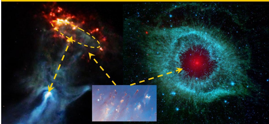
Figure 7, The A-symmetric B 1509-58 nebula , and symmetric Helix nebula as examples of the difference between Fermion- and non- inertial dark matter black hole Quantum Gravity effects.
