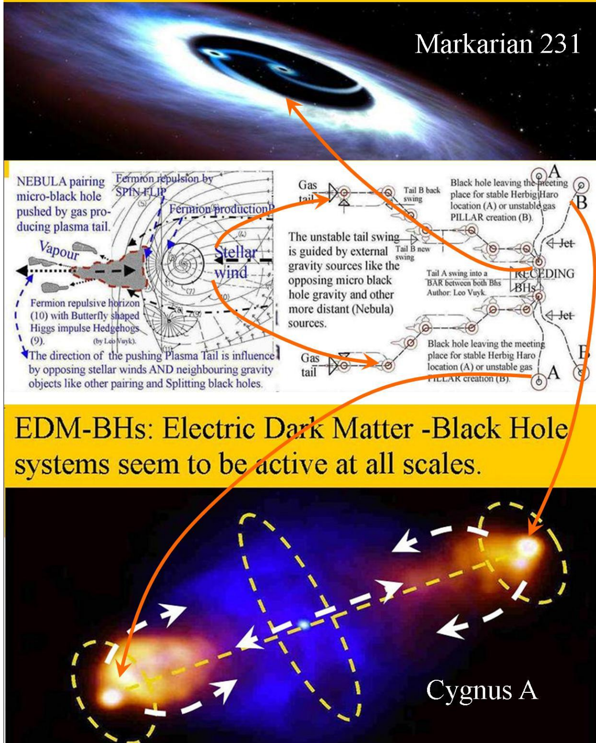
Figure 10. . the relation between Markarian 231 and other BH splitting systems
