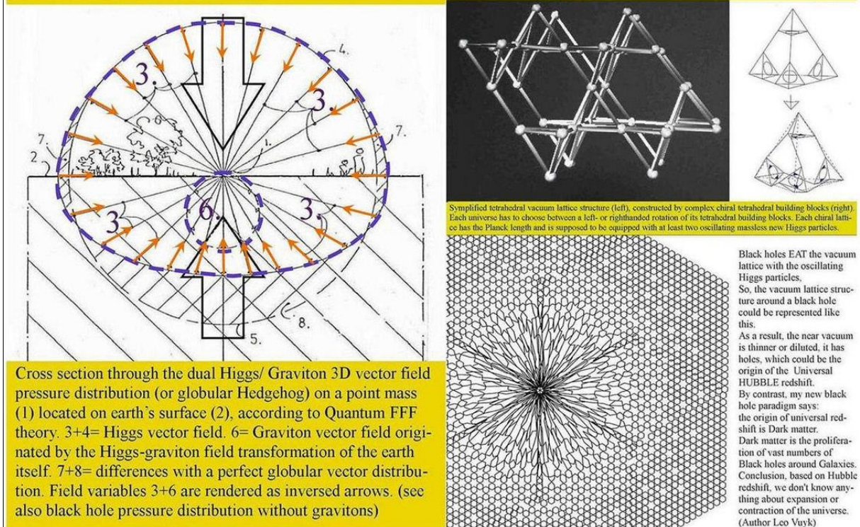
Figure 16, Quantum dipole repeller gravity ( the oscillating Casimir vacuum ) combined with less pressure from pushing gravitons.
