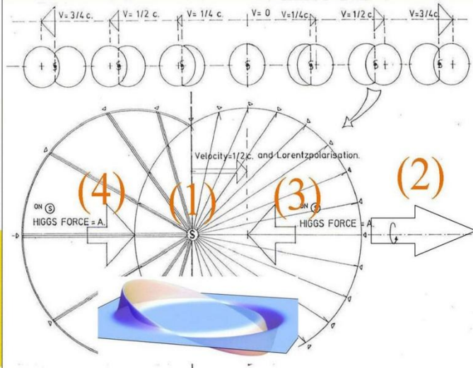
Figure 14, Quantum Gravity and Mass in motion. ( Quantum FFF Theory)
