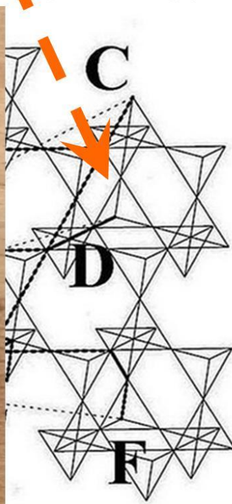
Figure 6, A stable black hole nucleus is large enough to “eat” the vacuum particles and grow by it.
