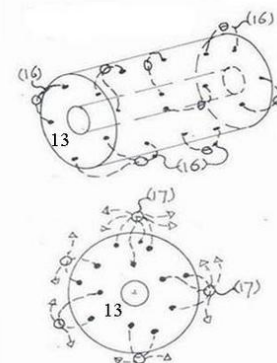
Figure 13 , BBBH , the Big Bang Black Hole splintering into smaller BHs and evaporating into the oscillating Axion Higgs Vacuum lattice .
