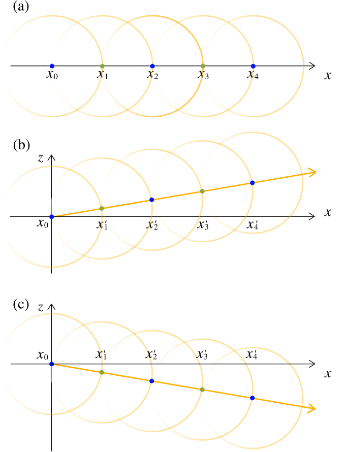
FIG. 7. (a) Linear motions of electrons when not receiving spin angular momentum. (b) and (c) The movements of electrons gaining an upward and downward spin angular momentum, respectively.
