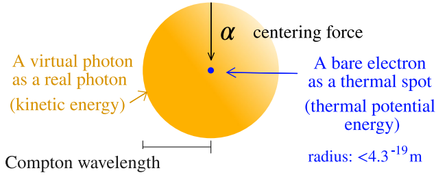
FIG. 8. Modified electron model
