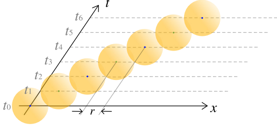
FIG. 2. Modified image of an electron in this study moving uni-directionally along the x axis. During each time interval t_n to t_{n+1} , the electron travels a distance r .
