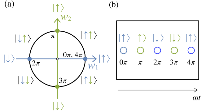
FIG. 3. a) One-state spin and an alternating two-state superposition of an electron's phase. (b) Diagram corresponding to the Slinky's footprints to the phases in (a).
