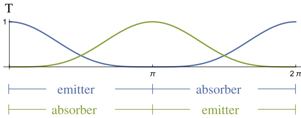
FIG. 9. Plots of T_{e1} = E_0 \cos^4(\frac{\omega t}{2}) (blue) and T_{e2} = E_0 \sin^4(\frac{\omega t}{2}) (green) with E_0 = 1 .
