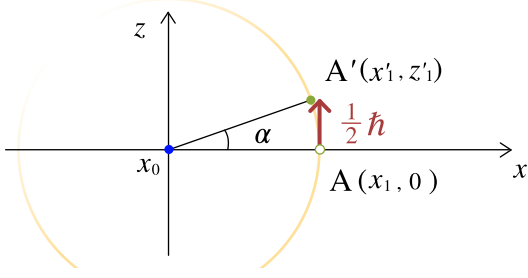
FIG. 4. From its point position at x_0 = 0 , t_0 = 0 (blue dot), the electron spreads to the Compton wavelength (yellow circle). At point A' , a bare electron has absorbed a photon in the phase \omega t = \pi . The green dot A'(x'_1, z'_1) is affected by the angular momentum.
