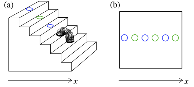
FIG. 1. (a) A Slinky painted blue and green on opposite sides moving down a stairway. (b) Footprints of the Slinky viewed from directly above the stairs.
