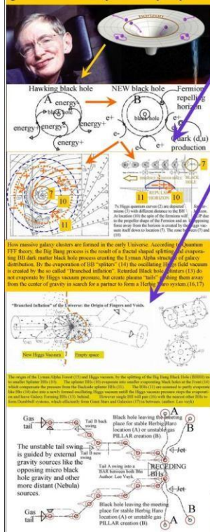
Figure 11, New paradigms according to Quantum FFF Theory.
