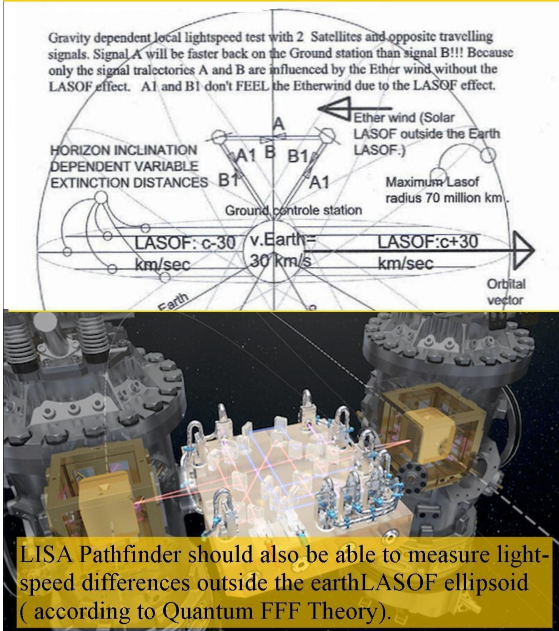
Figure 13, Gravity dependent lightspeed anomalies.
