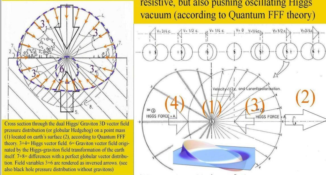
Figure 14, Quantum gravity.
