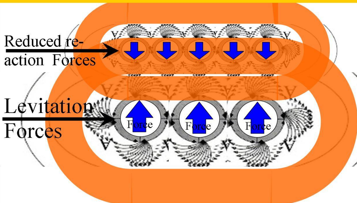
Figure 6, Levitation by dual conductor-conductor interference.
