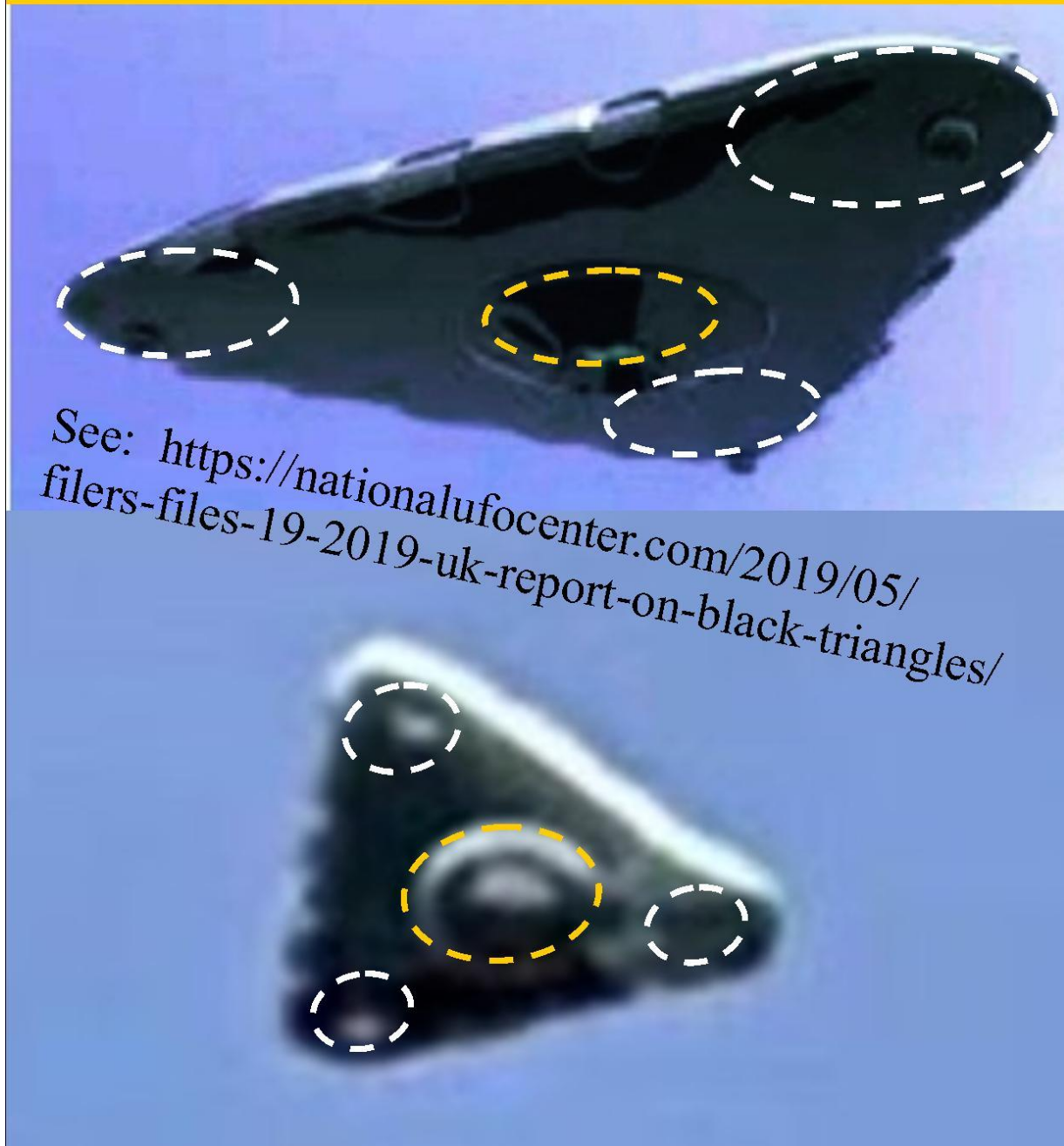
Figure 3, Three large EM drive discs seem to be here in action for levitation , or a combination of both small piloting rings inside larger levitation rings.
