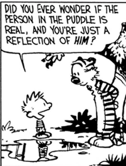
Figure 16, Anti matter deficit problem solved by mirror symmetric undivided ( entangled ) Multiverse without ead or alive Cats in boxes.
