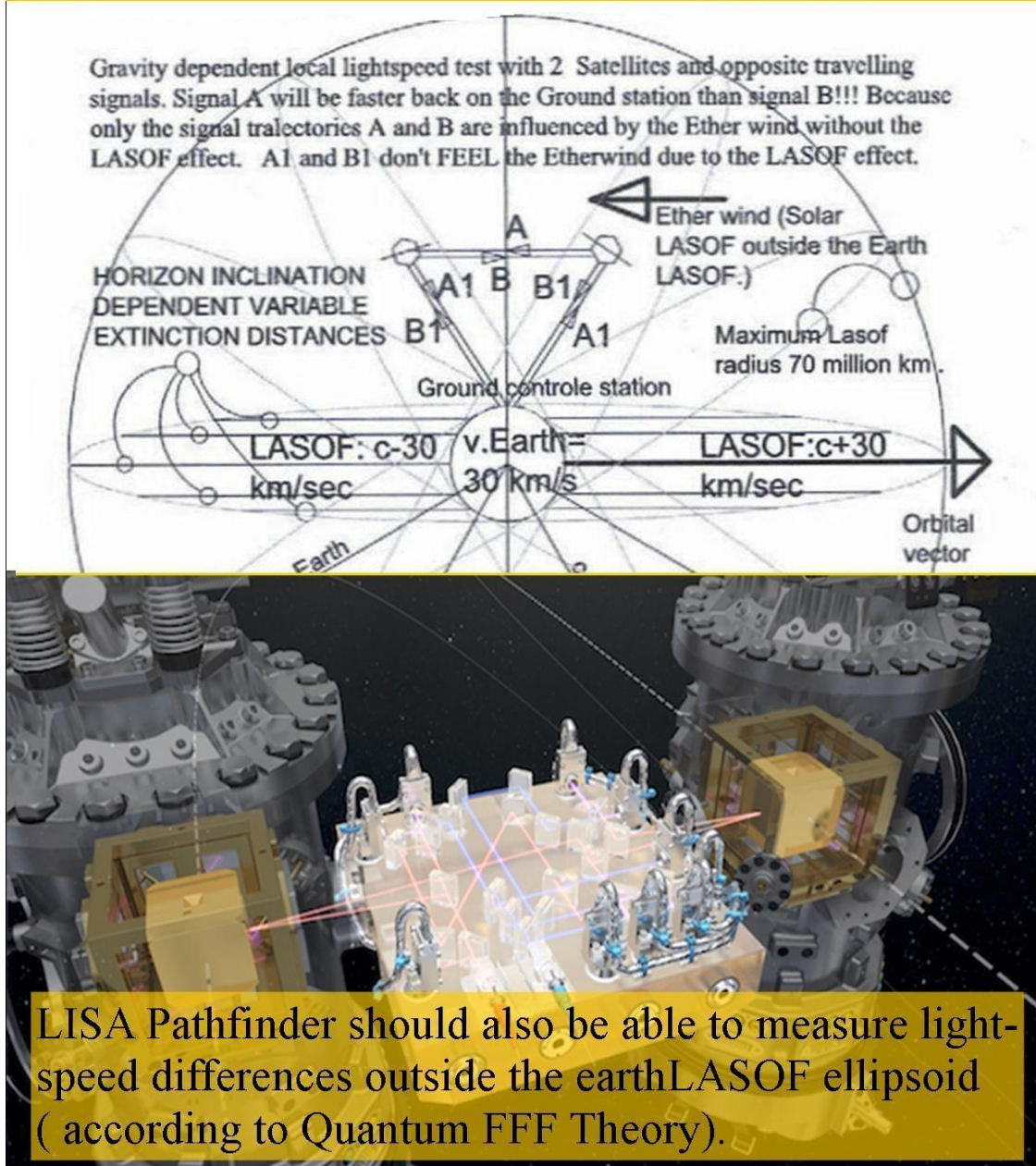
Figure 14, Gravity dependent lightspeed anomalies.
