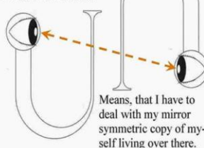
Figure 16, Anti matter deficit problem solved by mirror symmetric undivided ( entangled ) Multiverse without ead or alive Cats in boxes.
