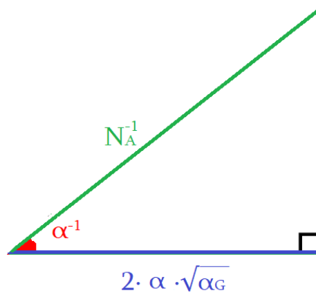
Figure 11. Second geometric representation of the simple unification of the gravitational and the electromagnetic interactions
