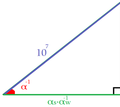
Figure 8. Geometric representation of the simple unification of the strong nuclear, the weak nuclear and the electromagnetic interactions.
