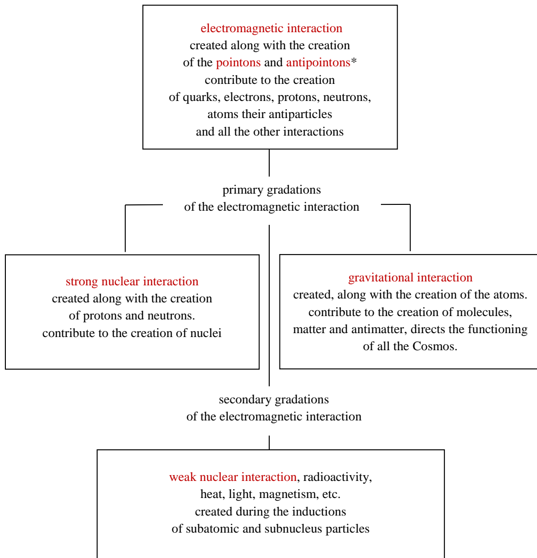
Diagram 2: The classification of the fundamental interactions according to the theory of the chain reaction
