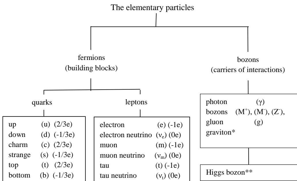
Diagram 1. The elementary particles according to the Standard Model theory
