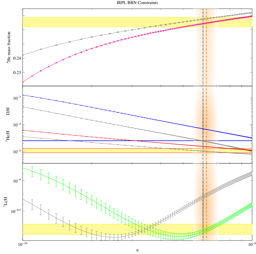
Figure 20. Comparison between the primordial abundances expected for the light nuclei according to the \Lambda CDM model, grey lines, and the IRPL model, coloured lines. Yellow horizontal rectangles show range of the uncertainties in the primordial abundances measured values. The orange vertical line indicates the value of \eta = 6.325 \pm 0.8 \times 10^{-10} deduced in the present IRPL analysis, the grey one \eta = 6.105 \pm 0.055 \times 10^{-10} for the \Lambda CDM model [13]. The values were calculated using the version 2 of AlterBBN software, an open public code for the calculation of the abundance of the elements from Big-Bang nucleosynthesis. For the purpose of the IRPL model, the bbnrate.c file was modified by adding the instruction “ f[ie]=0.5*f[ie]; ” at the end of the loop of the rate all function in order to halve all the reaction rates.
