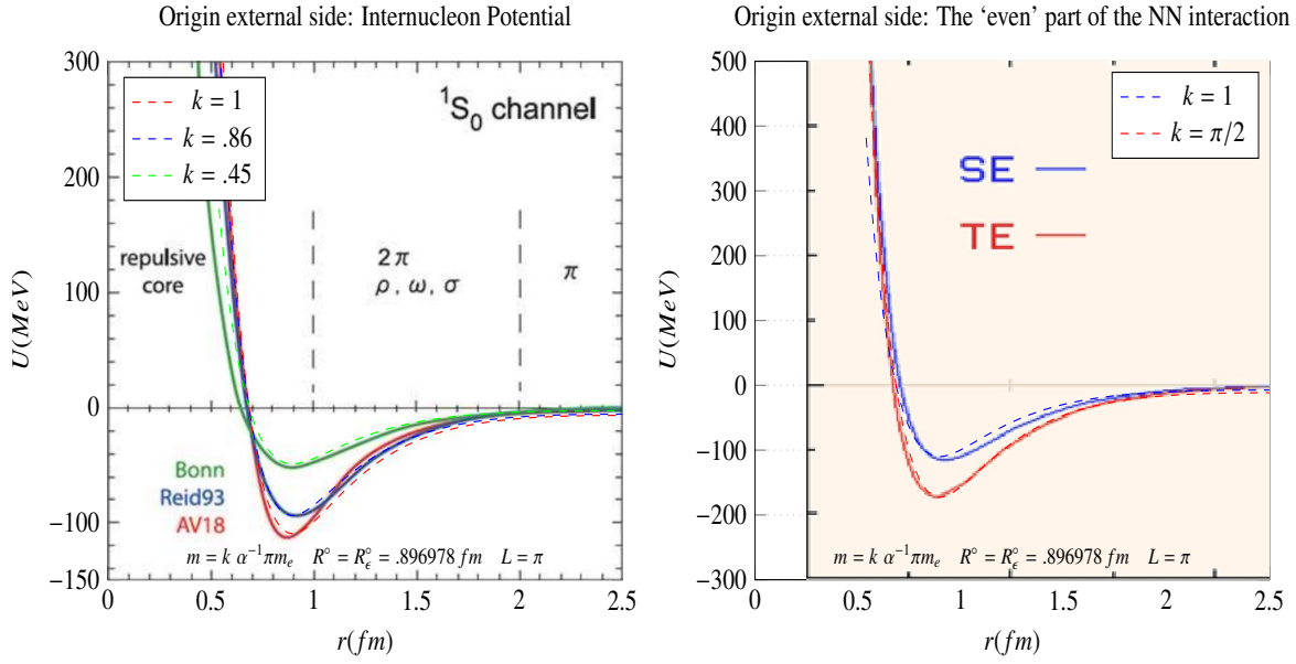
Figure 14. The internucleon potential comes from the external side of the strong area, where R^\circ = R_e^\circ = R_e^\circ/\pi = 0.896978 fm and the eq. (24d) is particularized as: U = mc^2 \left( -V^\circ + \frac{1}{2} V^{\circ 2} + \frac{1}{2} \frac{L^2}{c^2} \left( \frac{R^\circ}{r^\circ} \right)^2 (1 - V^\circ)^2 \right) . The potential V^\circ = \frac{R^\circ}{r^\circ} for r^\circ \geq R^\circ , V^\circ = \frac{r^\circ}{R^\circ} for r^\circ \leq R^\circ . The results are in good agreement with the experience, though neglecting spin-orbit and hyperfine structure terms.
