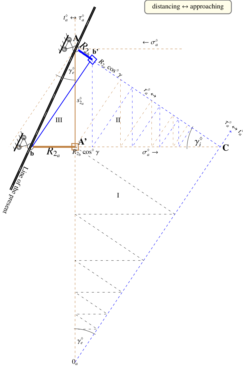
Figure 6. The whole relation is enfolds and unfolds from the Radii of the two conjoined individuals with the dual angles \gamma_e and \gamma_i alternating each other. It is governed by the relation V^\diamond = R_{tot} : r^\diamond = r^\diamond : \tau^\diamond = p^\diamond . That is, R_{tot} : CA = CA : OC or R_{tot} : A'C = A'C : OA' in distancing and R_{tot} : AC = AC : OA in approaching. Indeed the three quadrants represent time, space and Radius and recursively follow one another. In particular the III-II quadrants represent the internal energy-space plane, while the II-I quadrants the external space-time plane. The diagram represents the historical reconstruction of the relationship starting from the current instant. It coincides with real history only when \gamma is constant.
